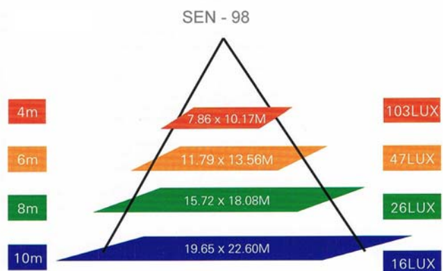
Isolux diagram
