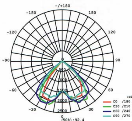
Spectrum chart
