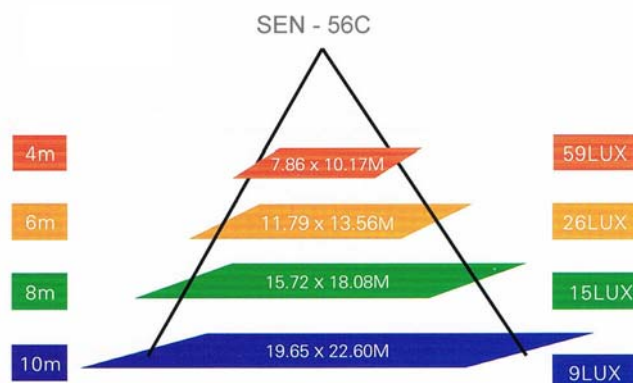
Isolux diagram
